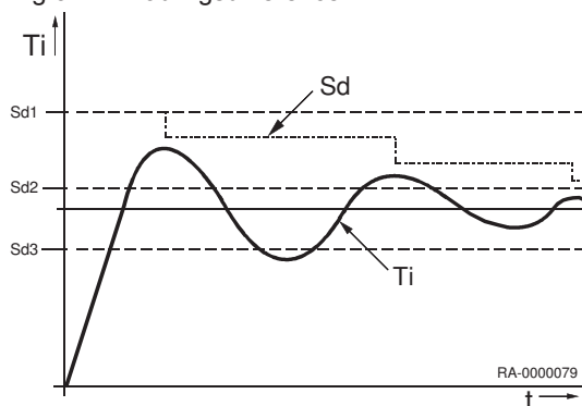
Fig.32 Koblingsdifferens
