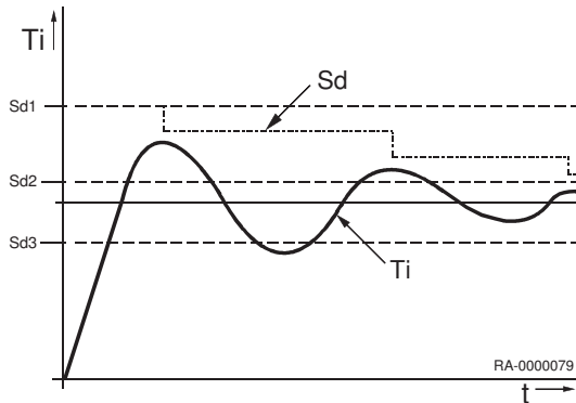
Fig.28 Koblingsdifference
