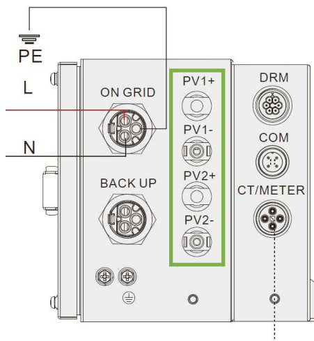
Ill. 4.2 - Inverteren har to MPP.
