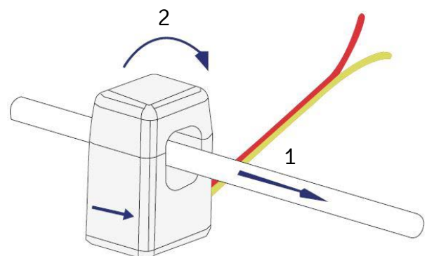
Ill. 5.3 - Montering af CT.
